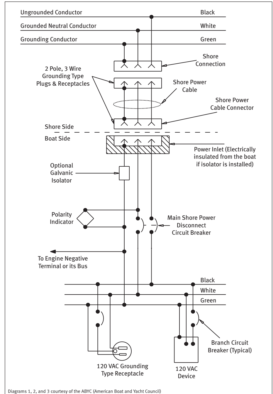
Diagram 1. Single-Phase 120 Volt System with Shore-Grounded Neutral Conductor and Grounding Conductor.
