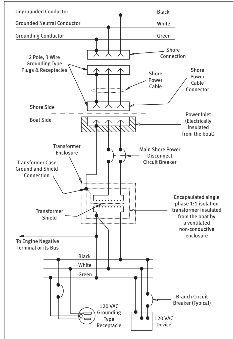
Diagram 3. Single-Phase 120 Volt Isolation Transformer System with Grounded Secondary.
